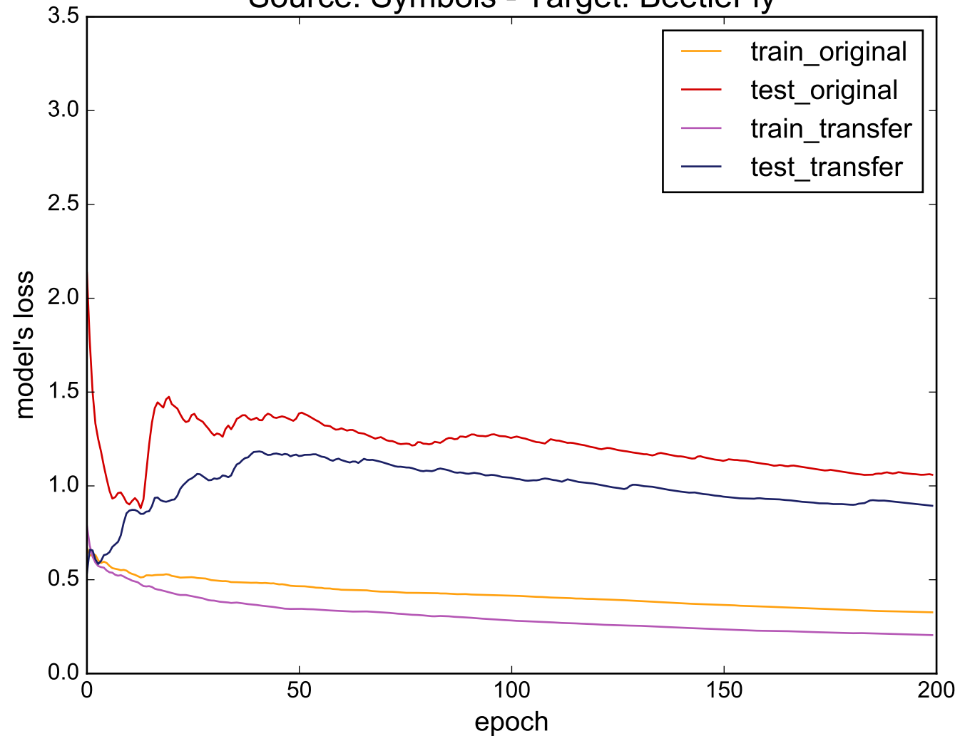
Source: Symbols - Target: BeetleFly
