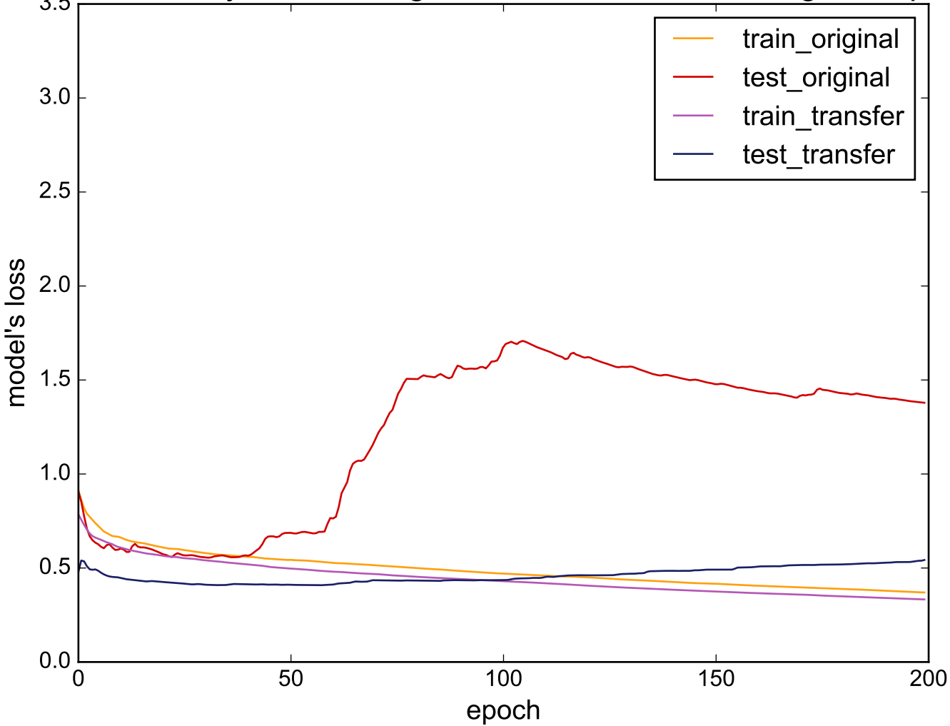
Source: Symbols - Target: DistalPhalanxOutlineAgeGroup
