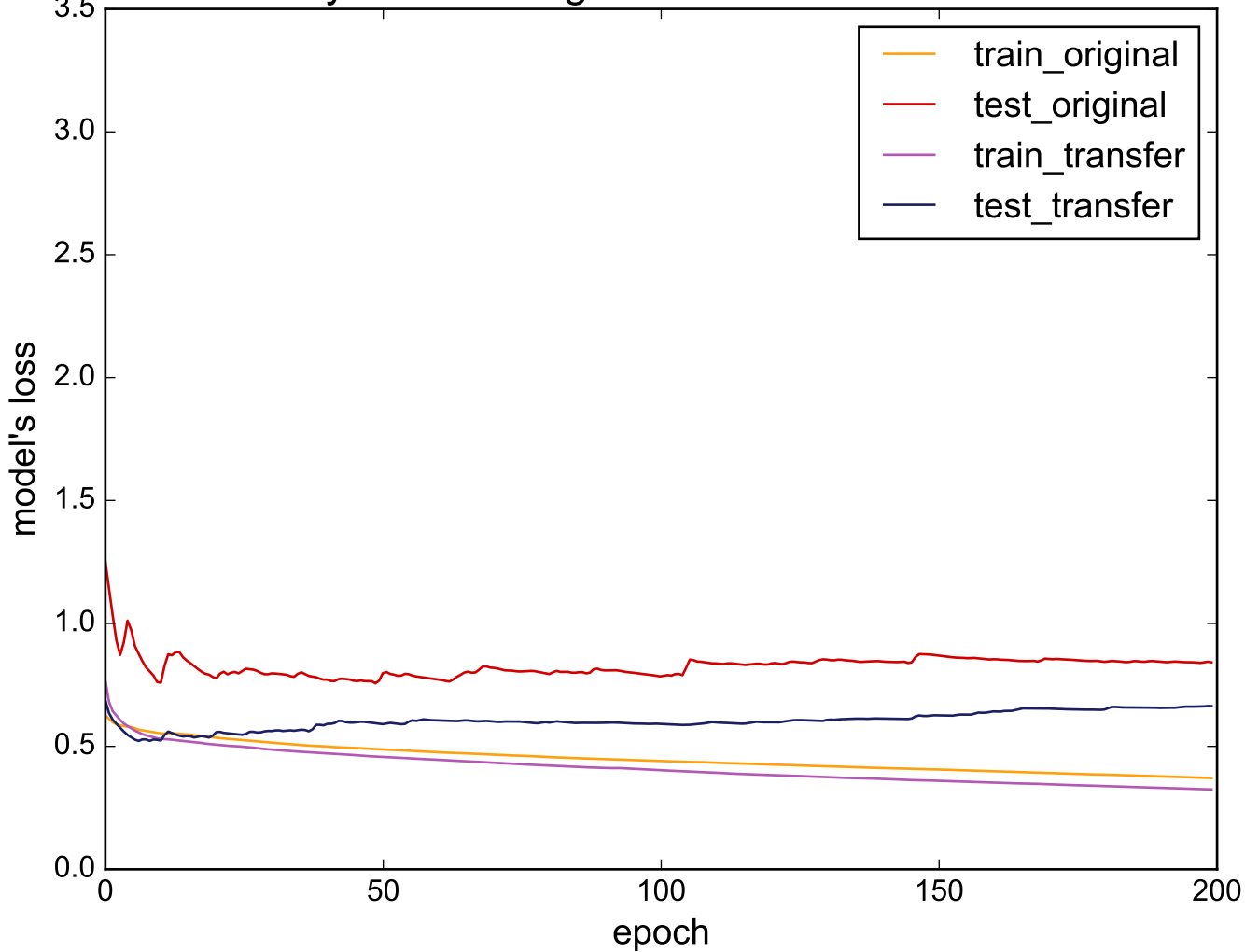
Source: Symbols - Target: DistalPhalanxOutlineCorrect
