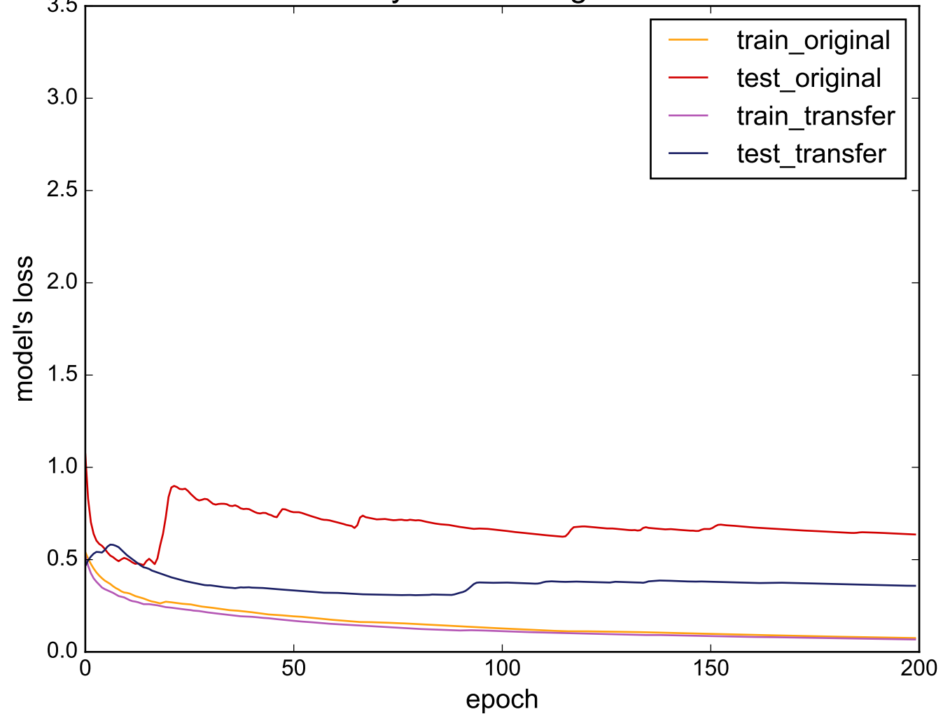
Source: Symbols - Target: ECG200
