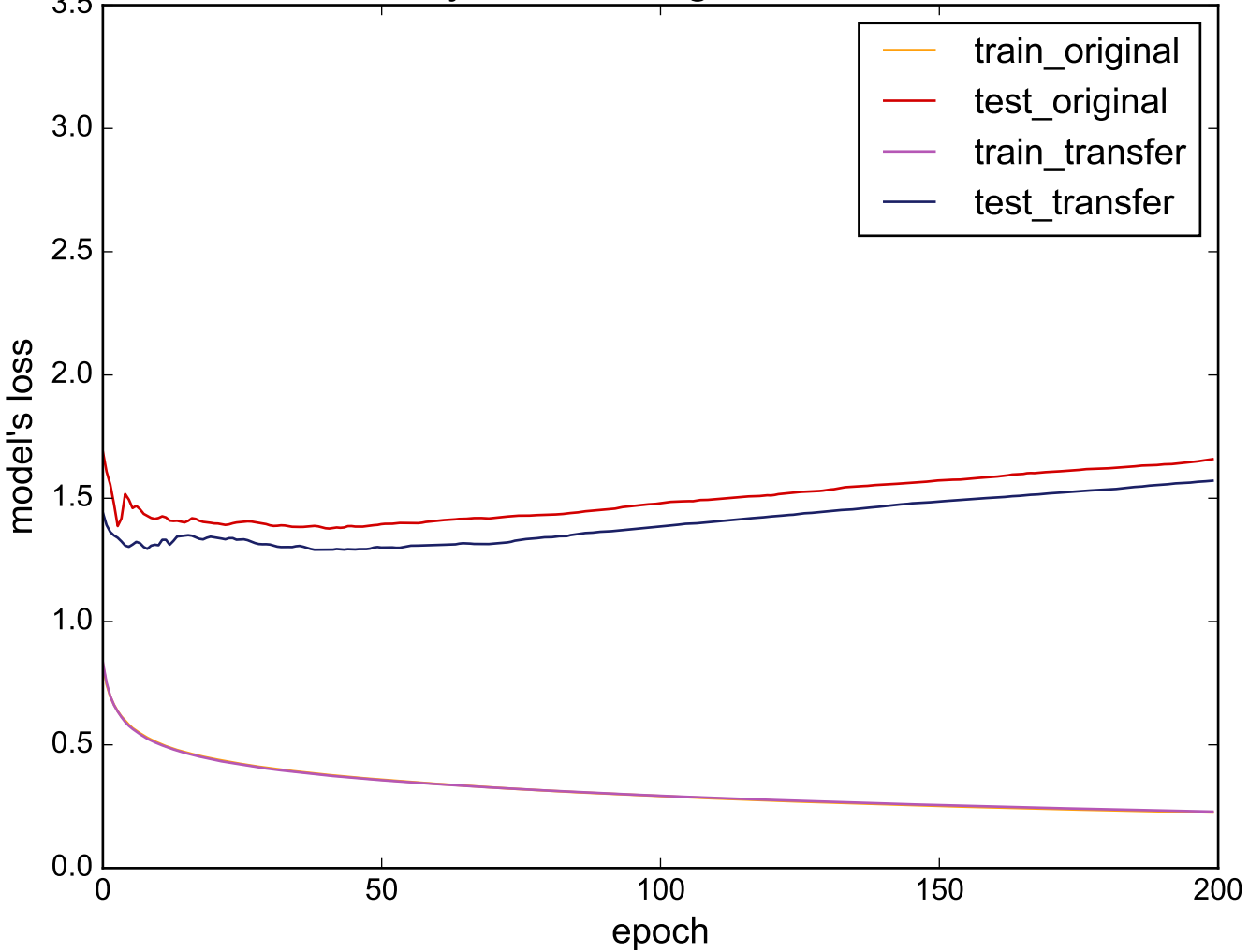
Source: Symbols - Target: ElectricDevices
