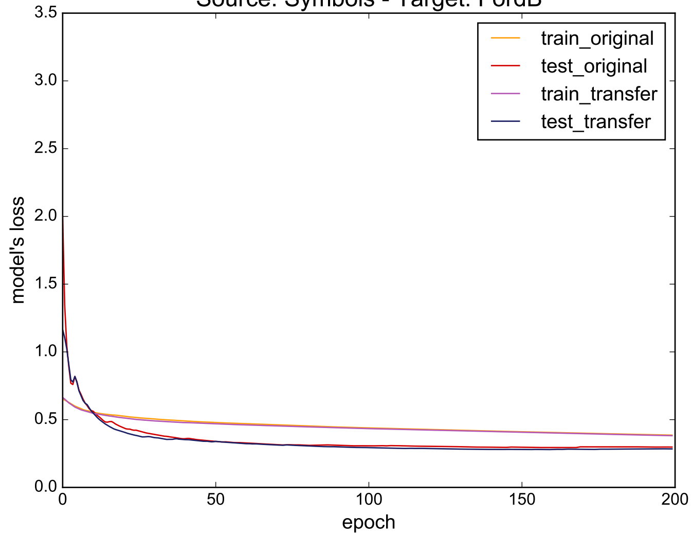
Source: Symbols - Target: FordB
