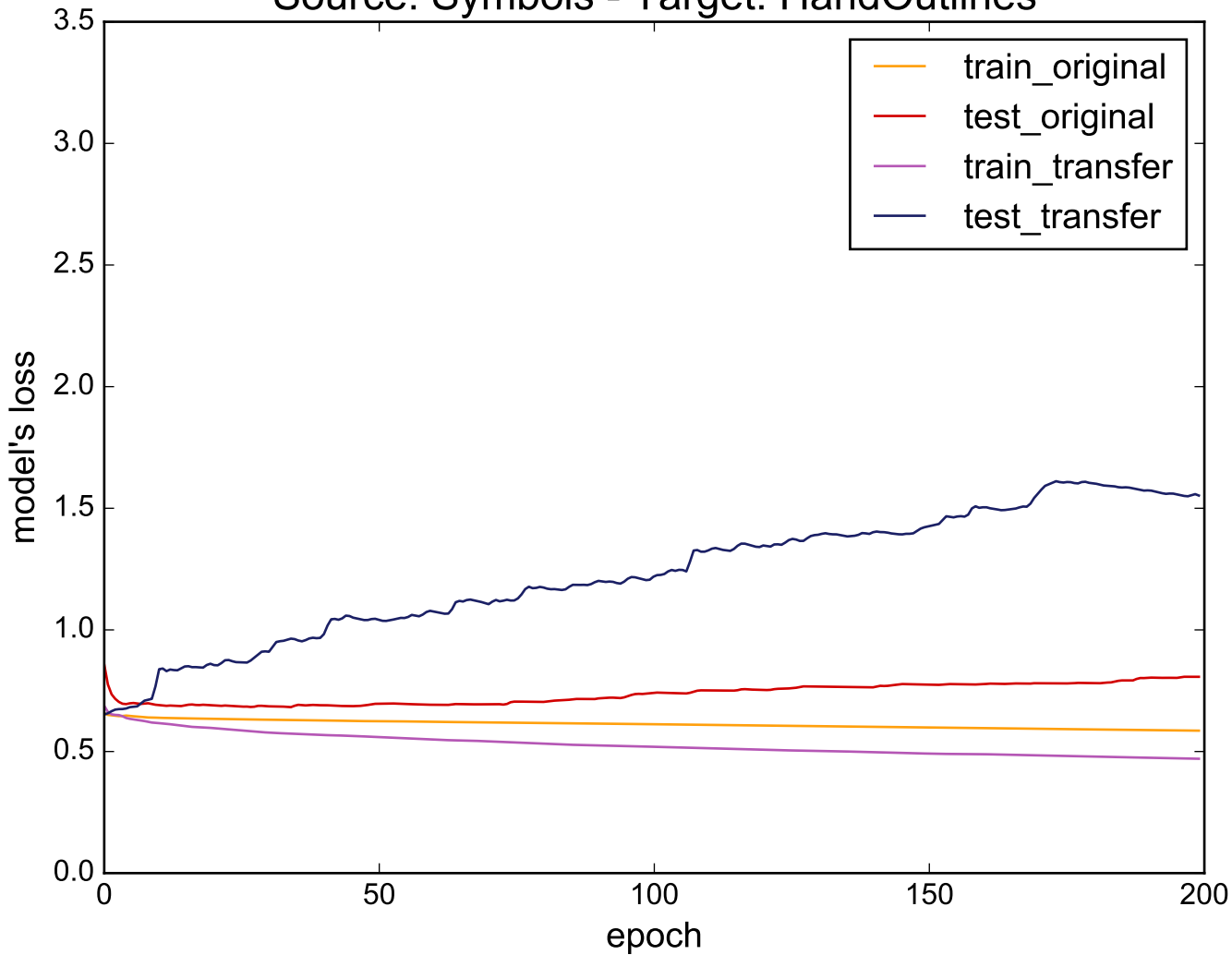
Source: Symbols - Target: HandOutlines
