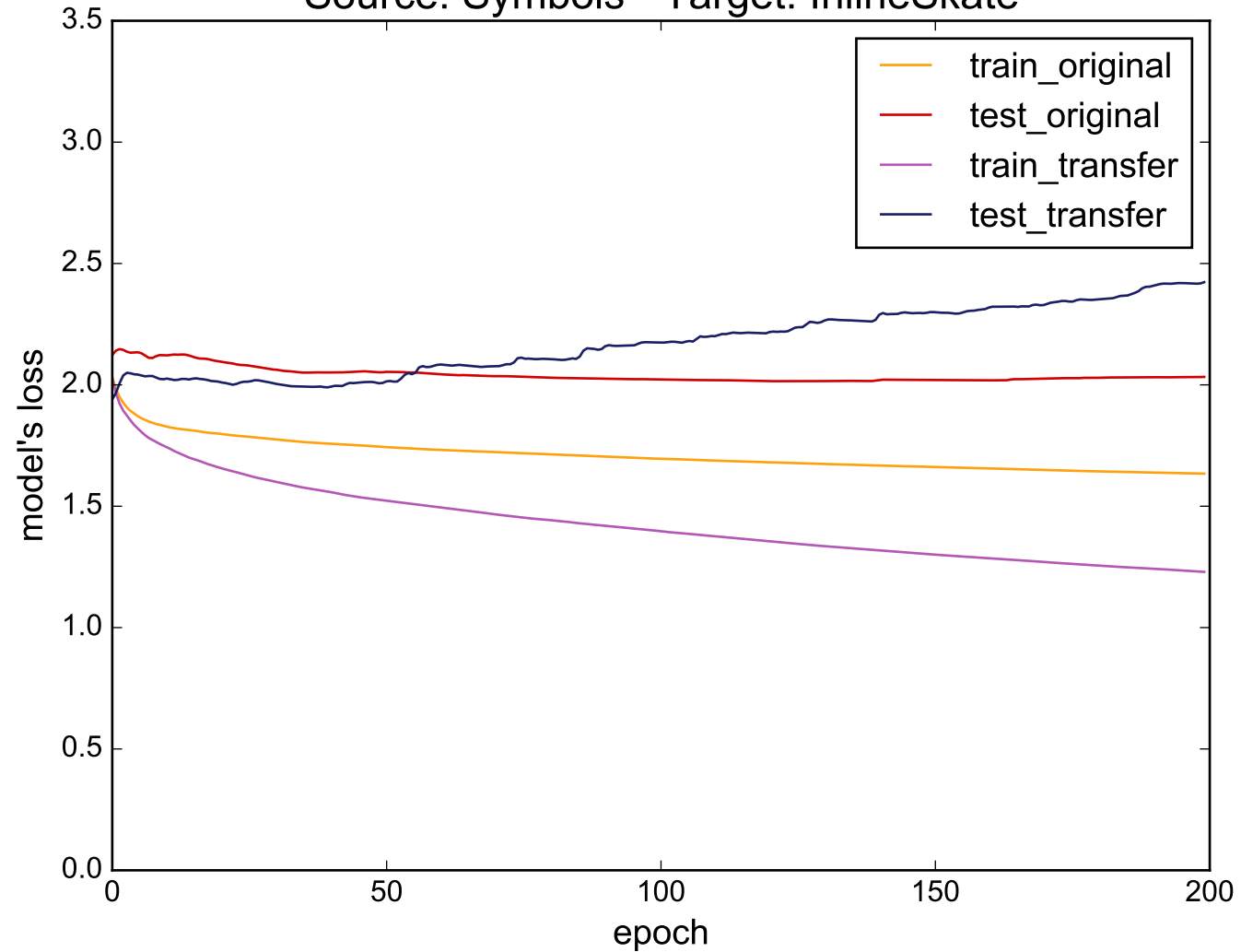
Source: Symbols - Target: InlineSkate
