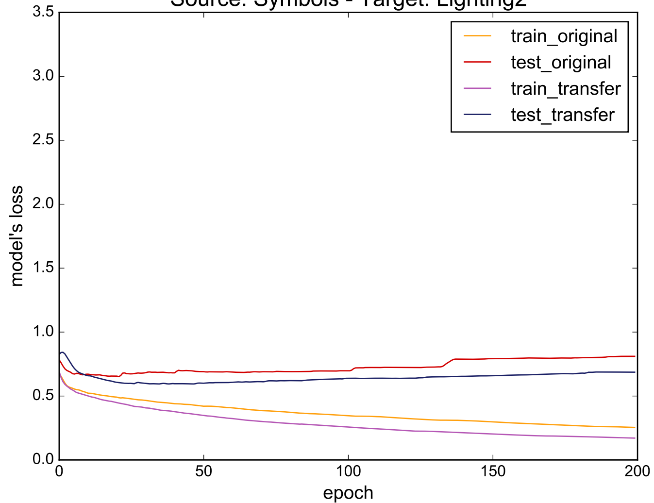
Source: Symbols - Target: Lighting2
