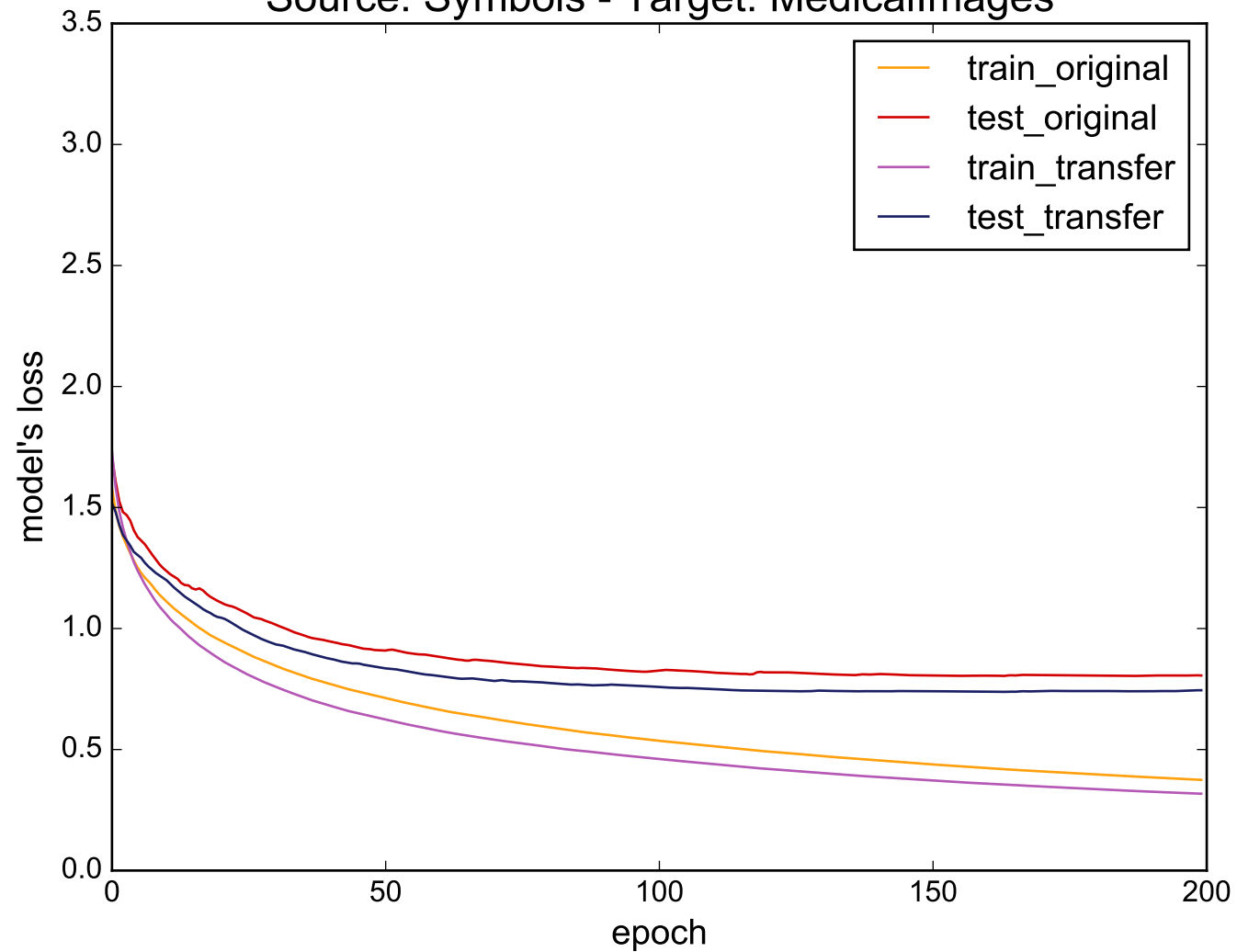
Source: Symbols - Target: MedicalImages
