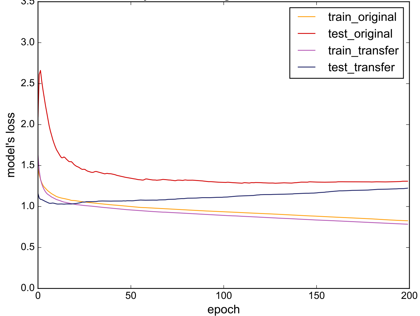
Source: Symbols - Target: MiddlePhalanxTW
