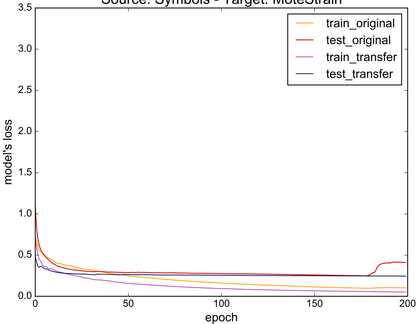
Source: Symbols - Target: MoteStrain
