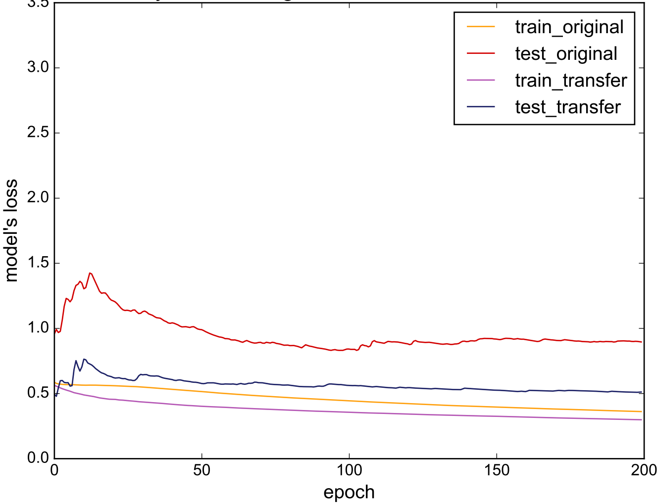
Source: Symbols - Target: ProximalPhalanxOutlineCorrect
