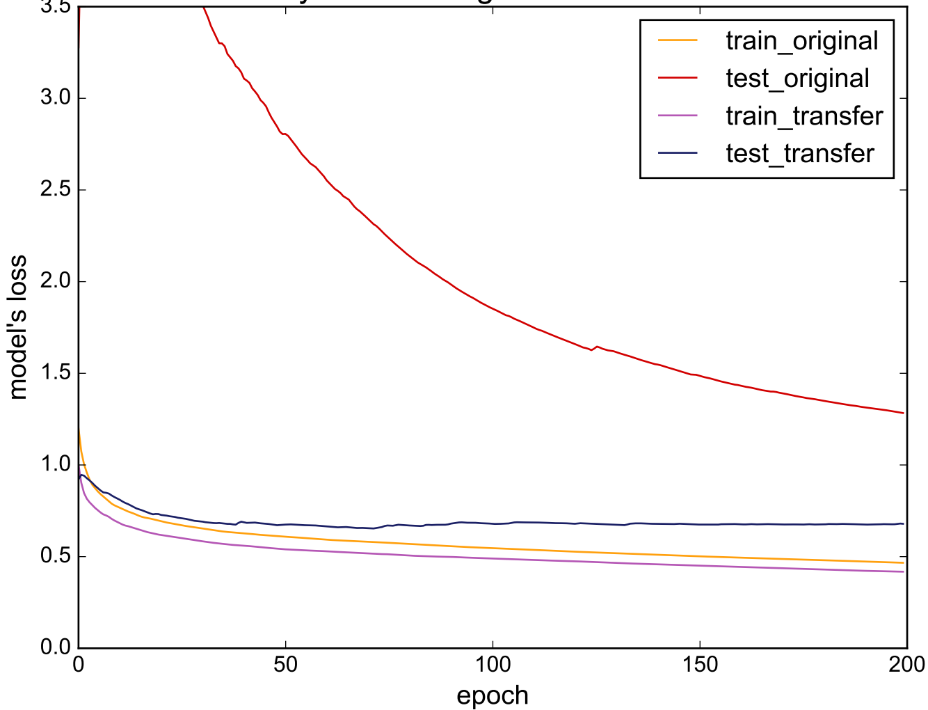
Source: Symbols - Target: ProximalPhalanxTW
