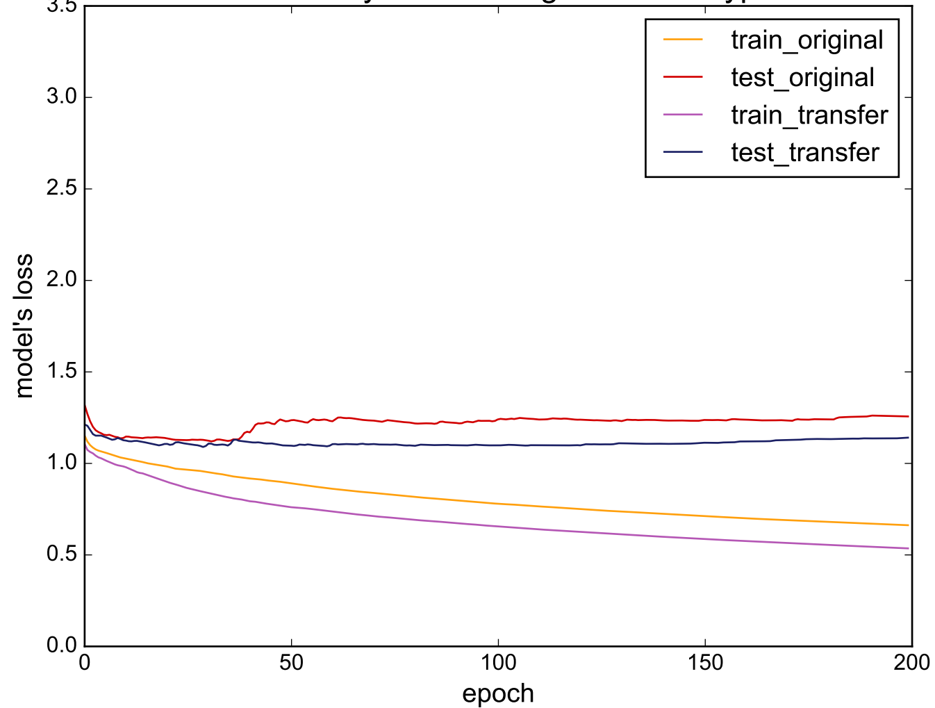
Source: Symbols - Target: ScreenType
