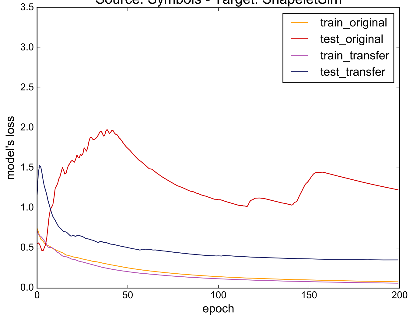
Source: Symbols - Target: ShapeletSim
