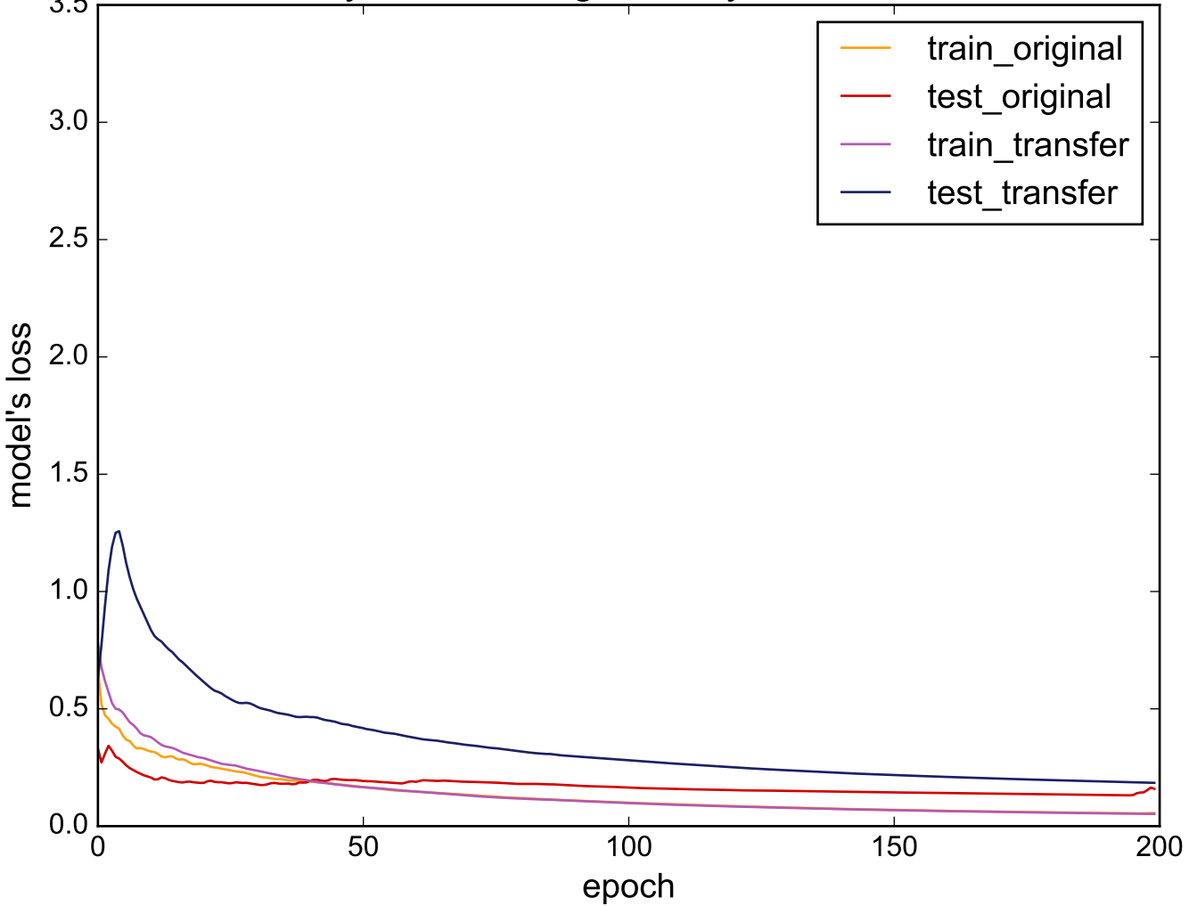
Source: Symbols - Target: SonyAIBORobotSurface
