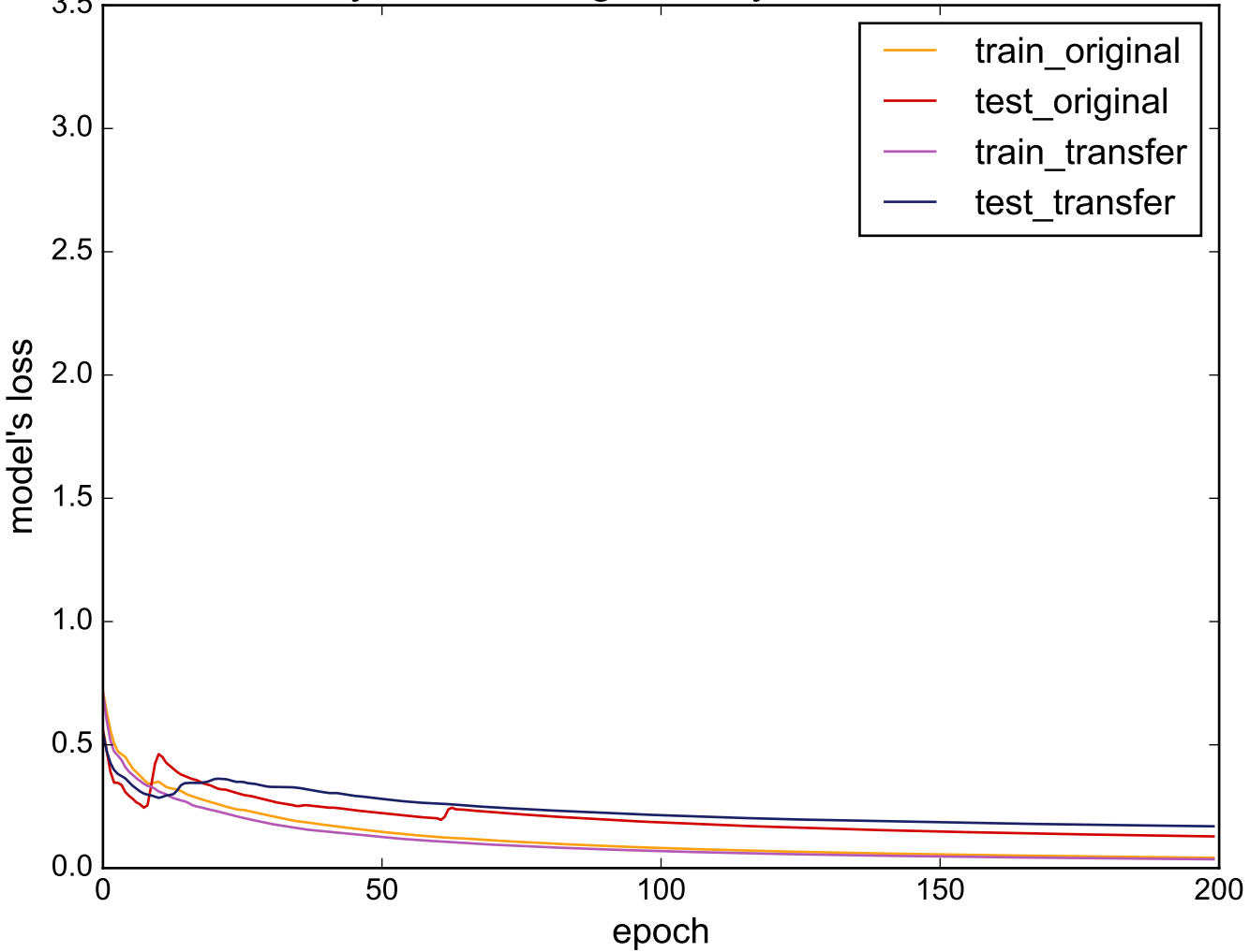
Source: Symbols - Target: SonyAIBORobotSurfaceII
