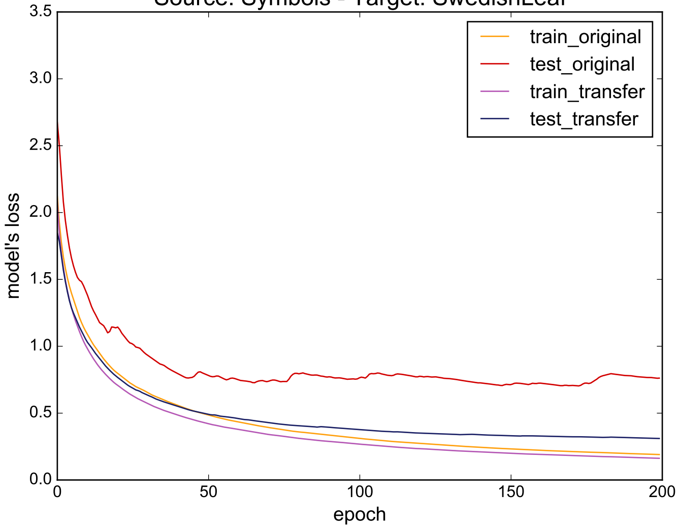
Source: Symbols - Target: SwedishLeaf
