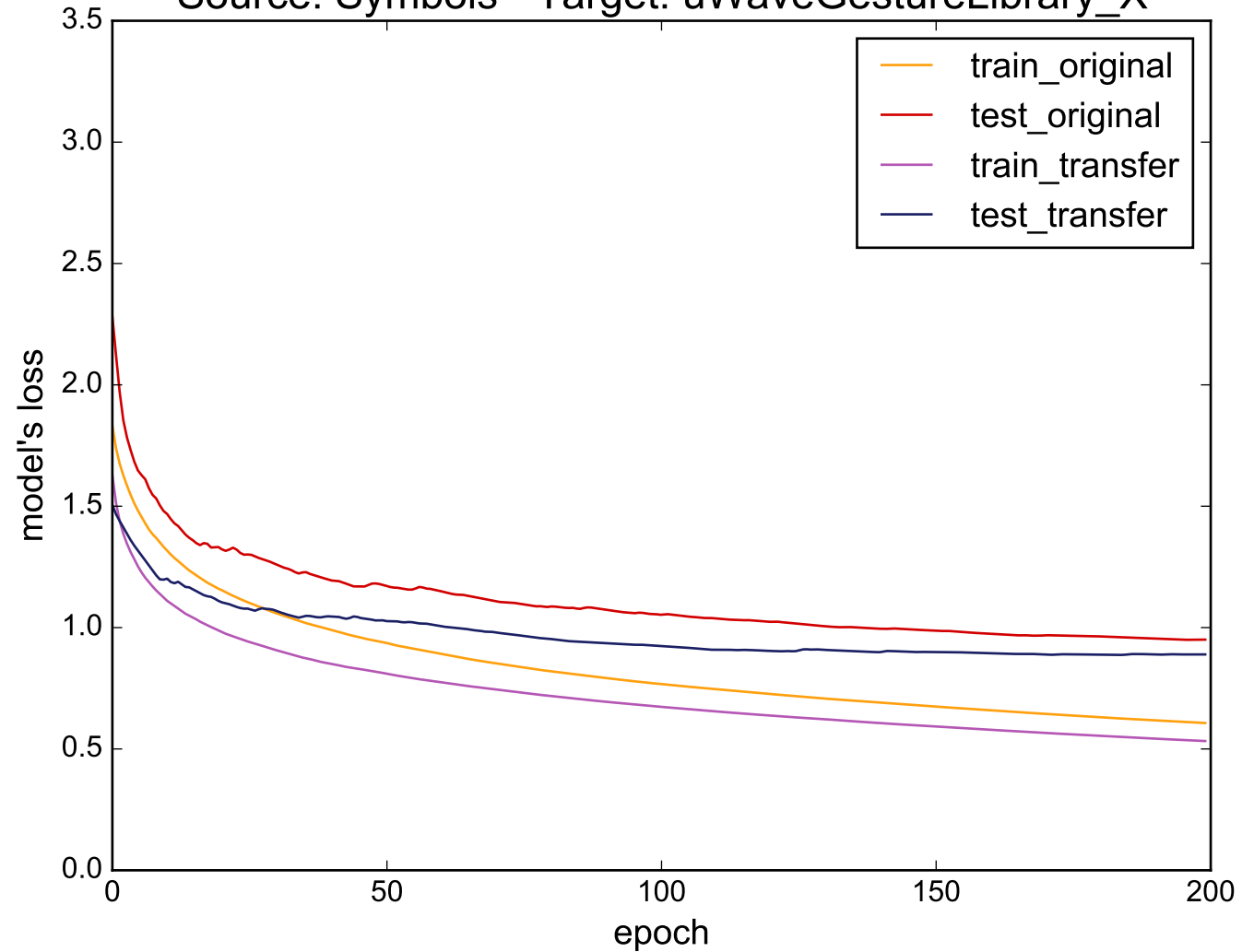
Source: Symbols - Target: uWaveGestureLibrary_X
