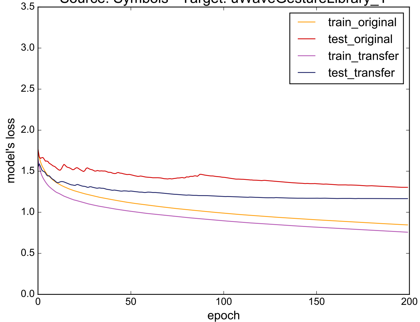
Source: Symbols - Target: uWaveGestureLibrary_Y
