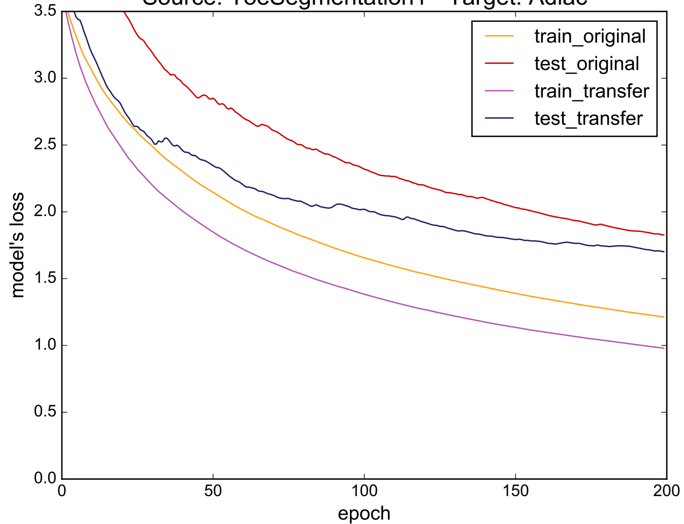
Source: ToeSegmentation1 - Target: Adiac
