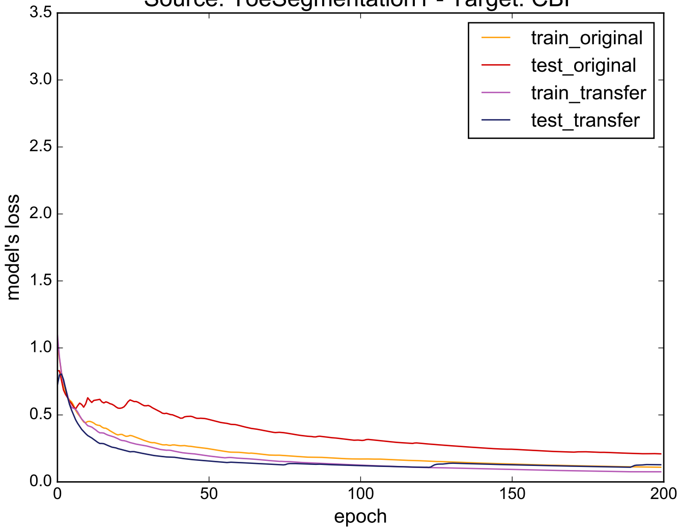
Source: ToeSegmentation1 - Target: CBF
