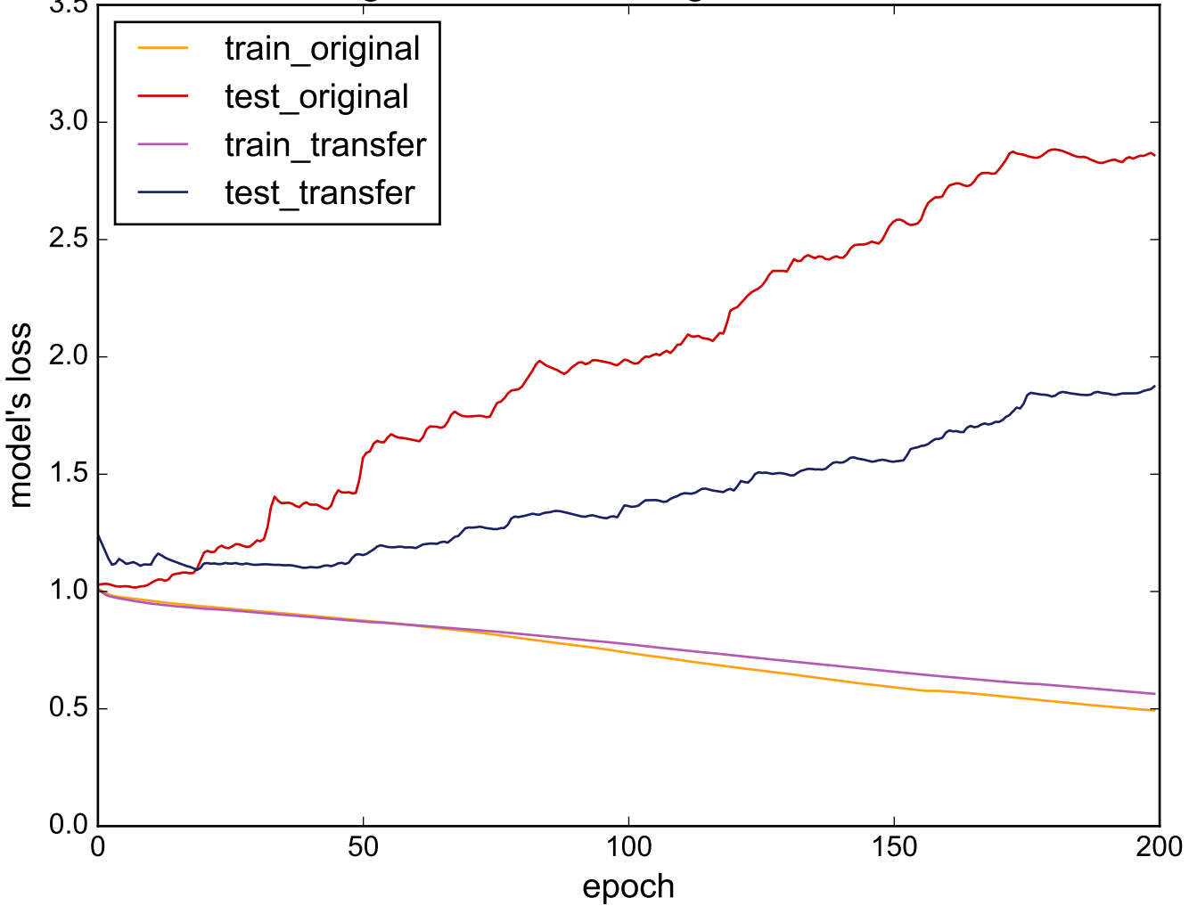
Source: ToeSegmentation1 - Target: ChlorineConcentration
