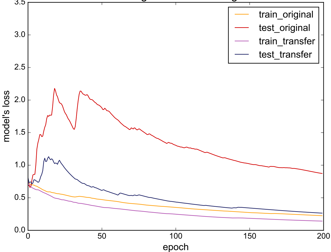
Source: ToeSegmentation1 - Target: Coffee
