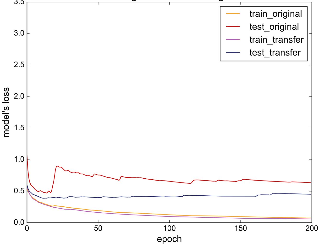
Source: ToeSegmentation1 - Target: ECG200
