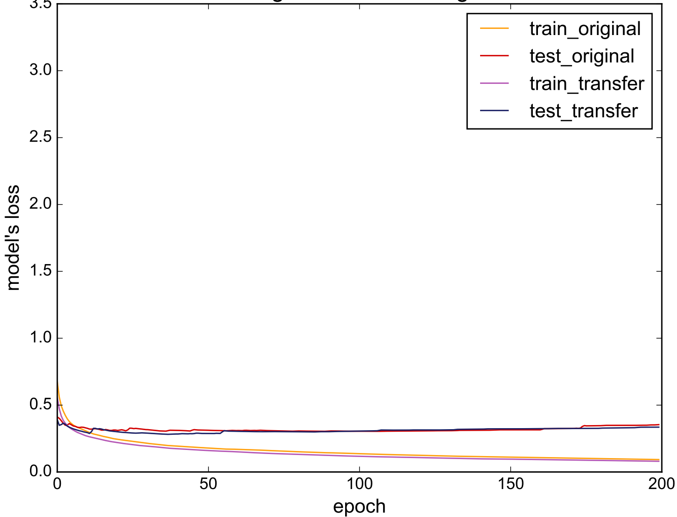
Source: ToeSegmentation1 - Target: ECG5000
