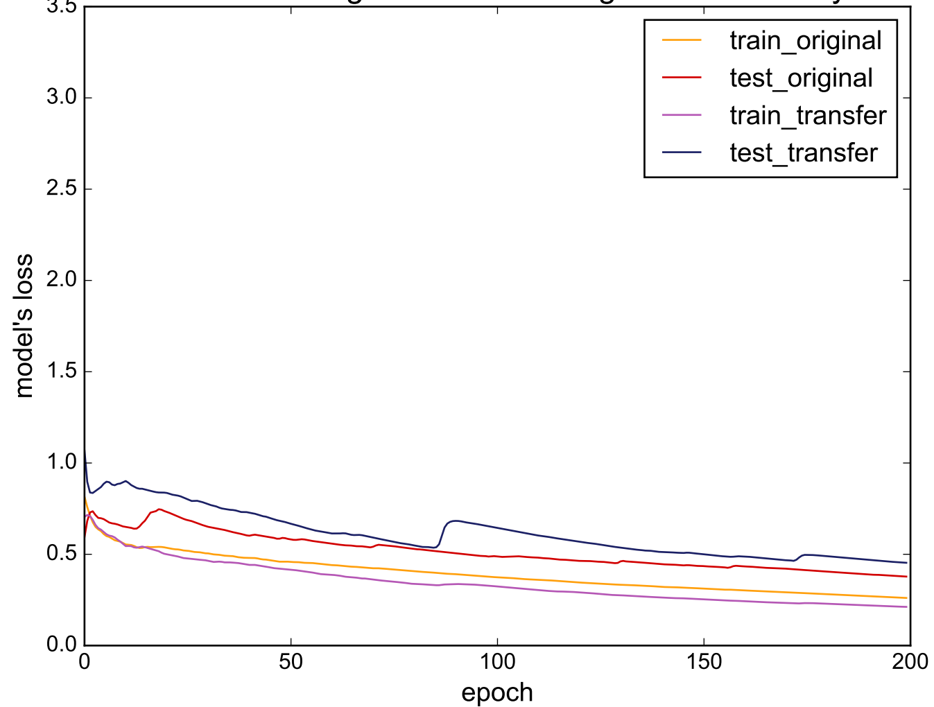
Source: ToeSegmentation1 - Target: ECGFiveDays
