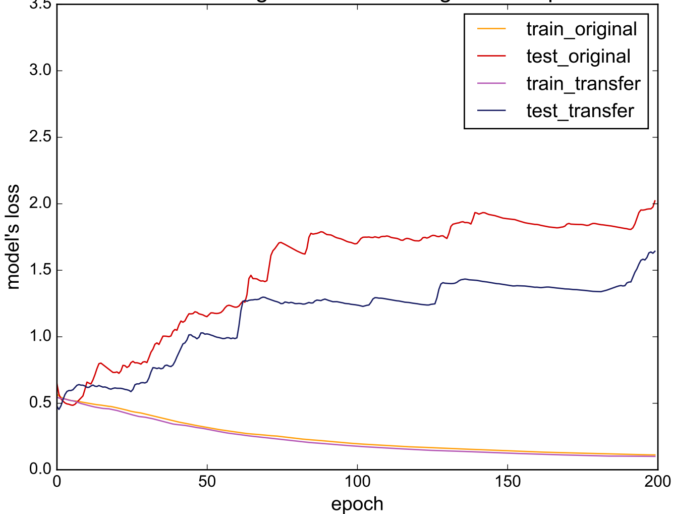
Source: ToeSegmentation1 - Target: Earthquakes
