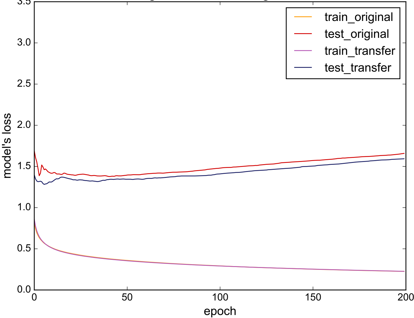
Source: ToeSegmentation1 - Target: ElectricDevices
