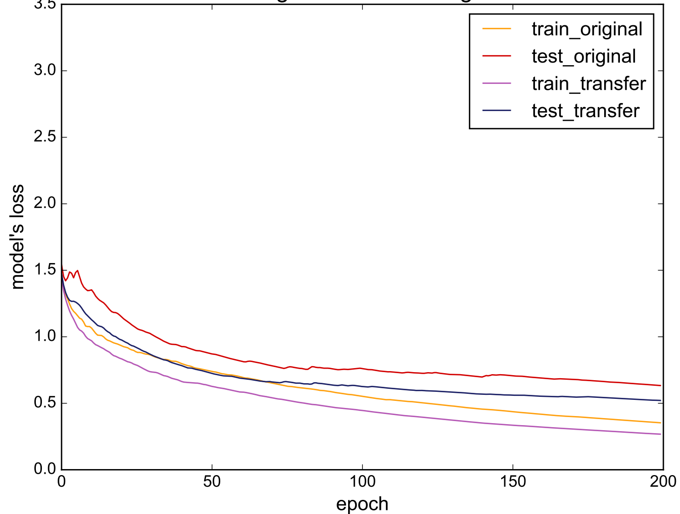
Source: ToeSegmentation1 - Target: FaceFour
