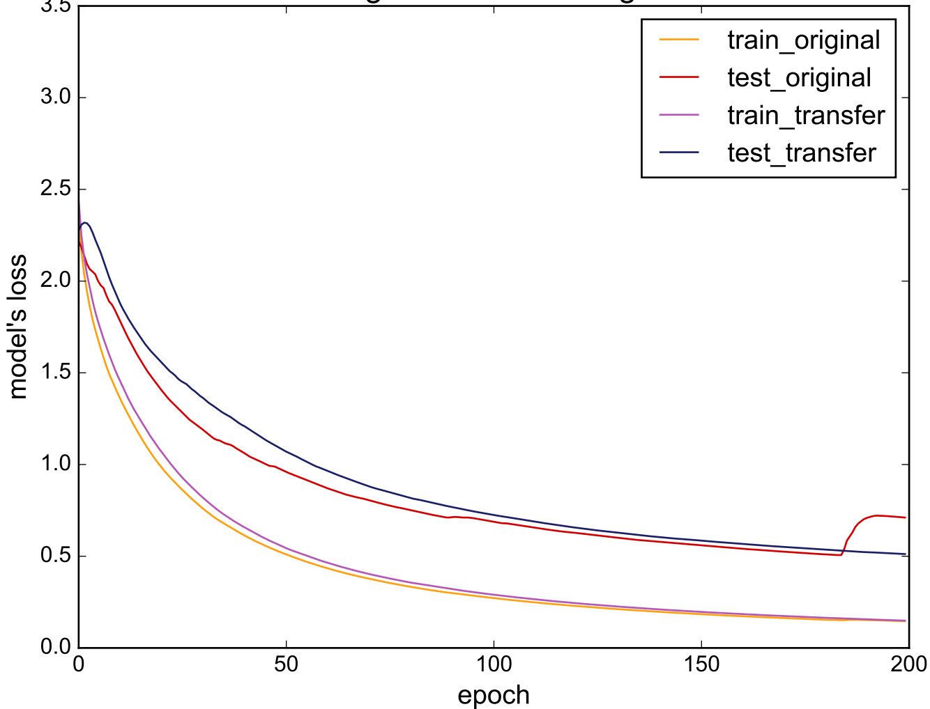
Source: ToeSegmentation1 - Target: FacesUCR
