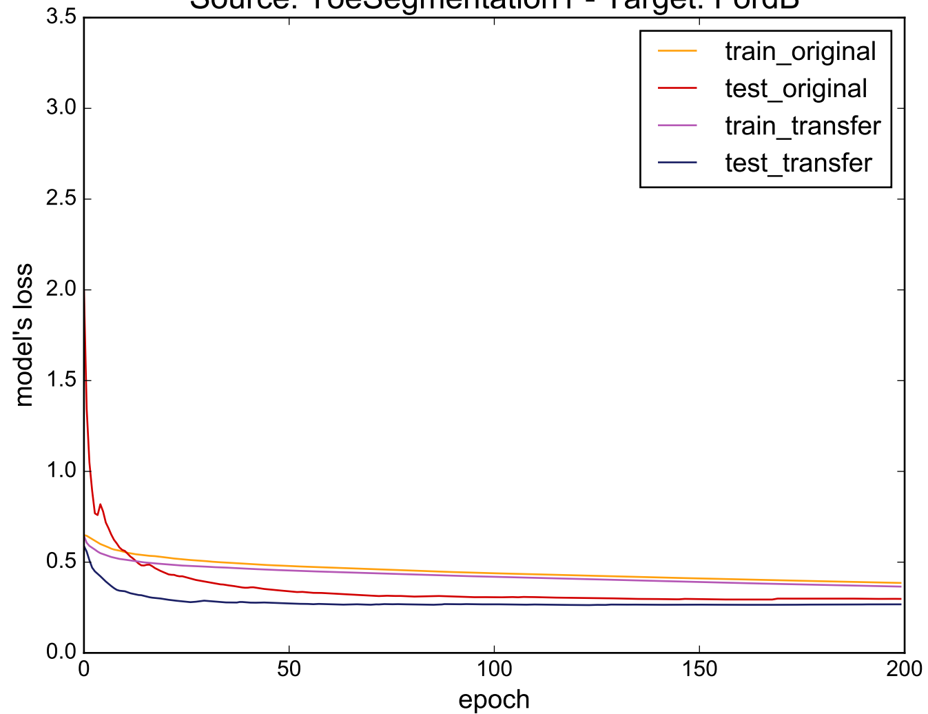
Source: ToeSegmentation1 - Target: FordB
