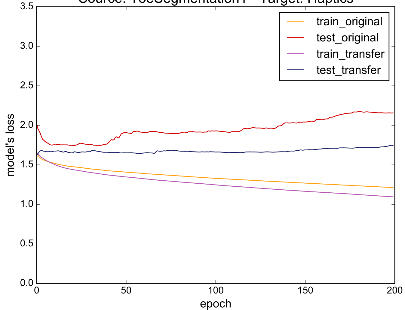
Source: ToeSegmentation1 - Target: Haptics
