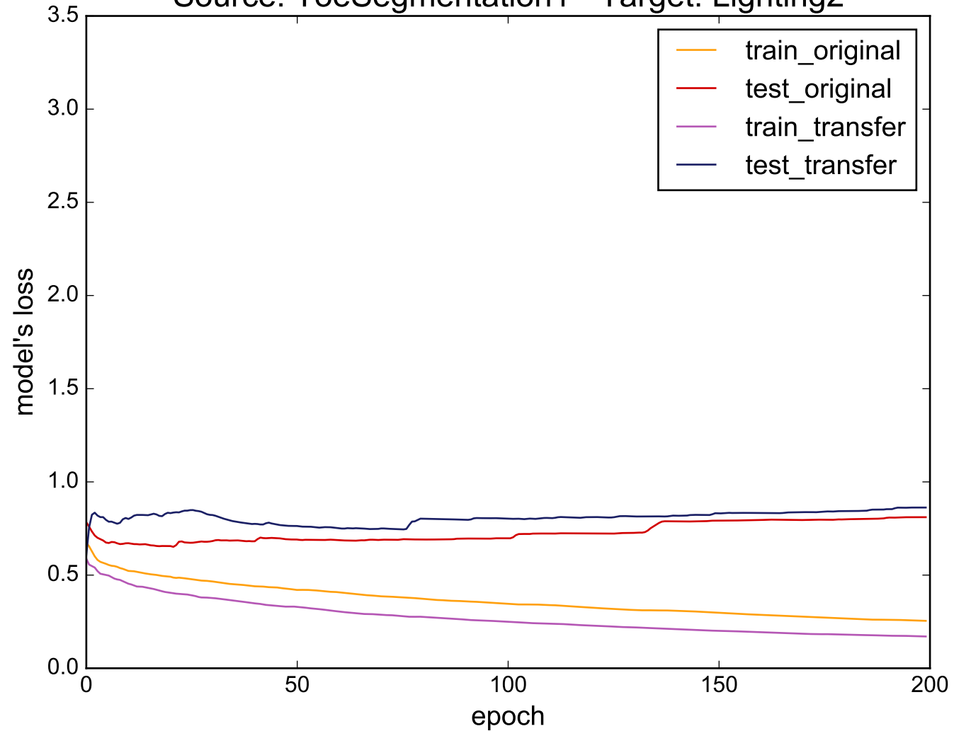
Source: ToeSegmentation1 - Target: Lighting2
