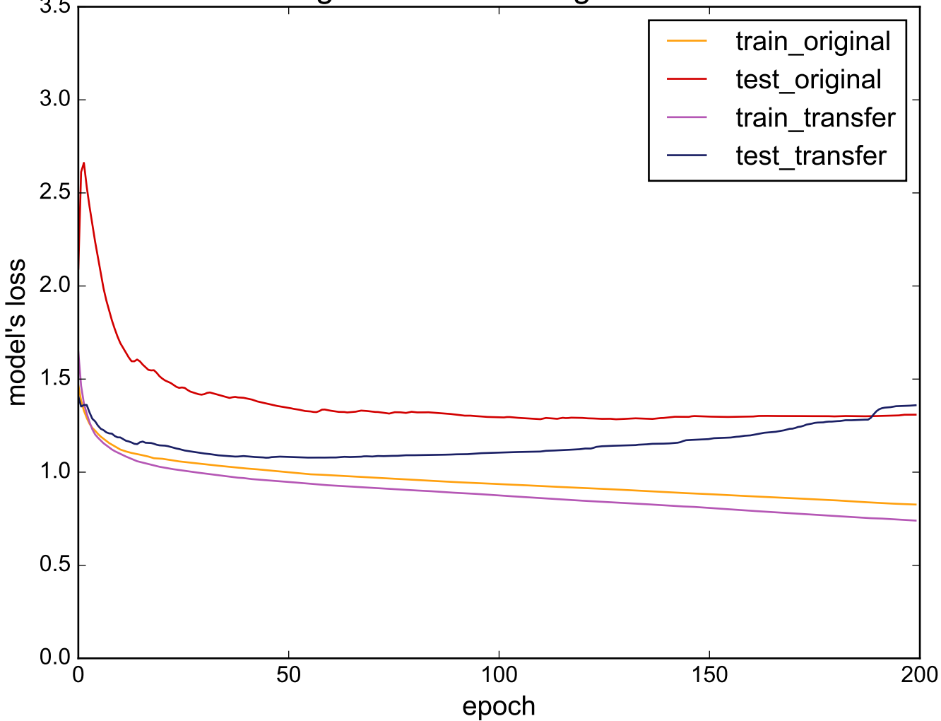
Source: ToeSegmentation1 - Target: MiddlePhalanxTW
