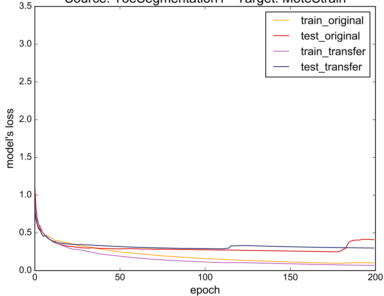
Source: ToeSegmentation1 - Target: MoteStrain
