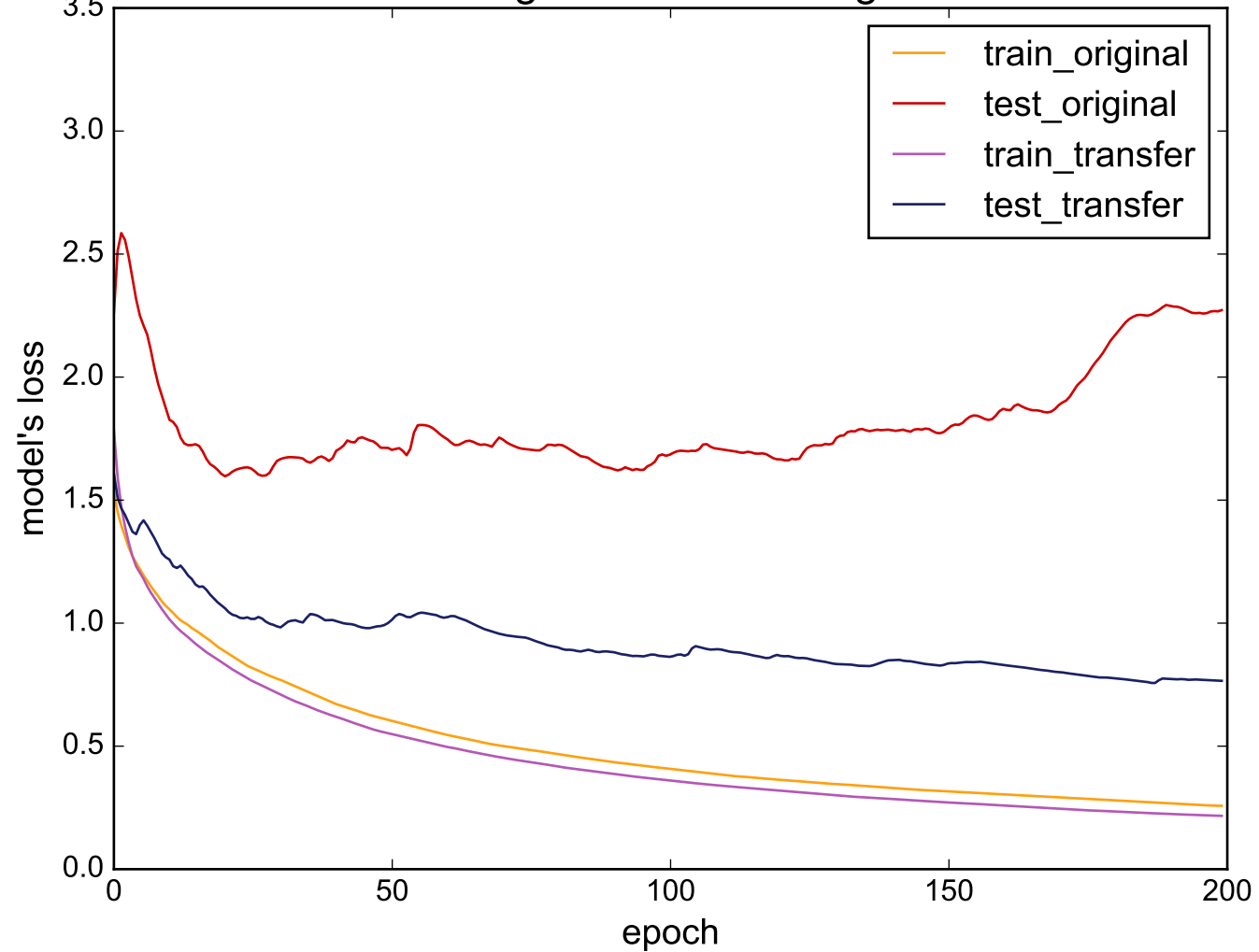
Source: ToeSegmentation1 - Target: OSULeaf
