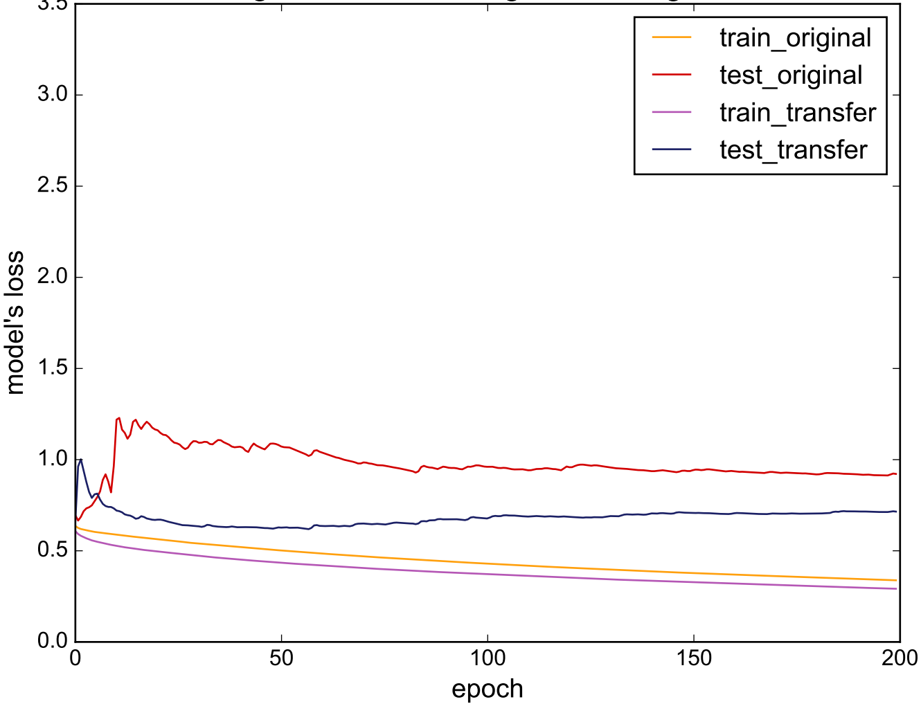
Source: ToeSegmentation1 - Target: PhalangesOutlinesCorrect
