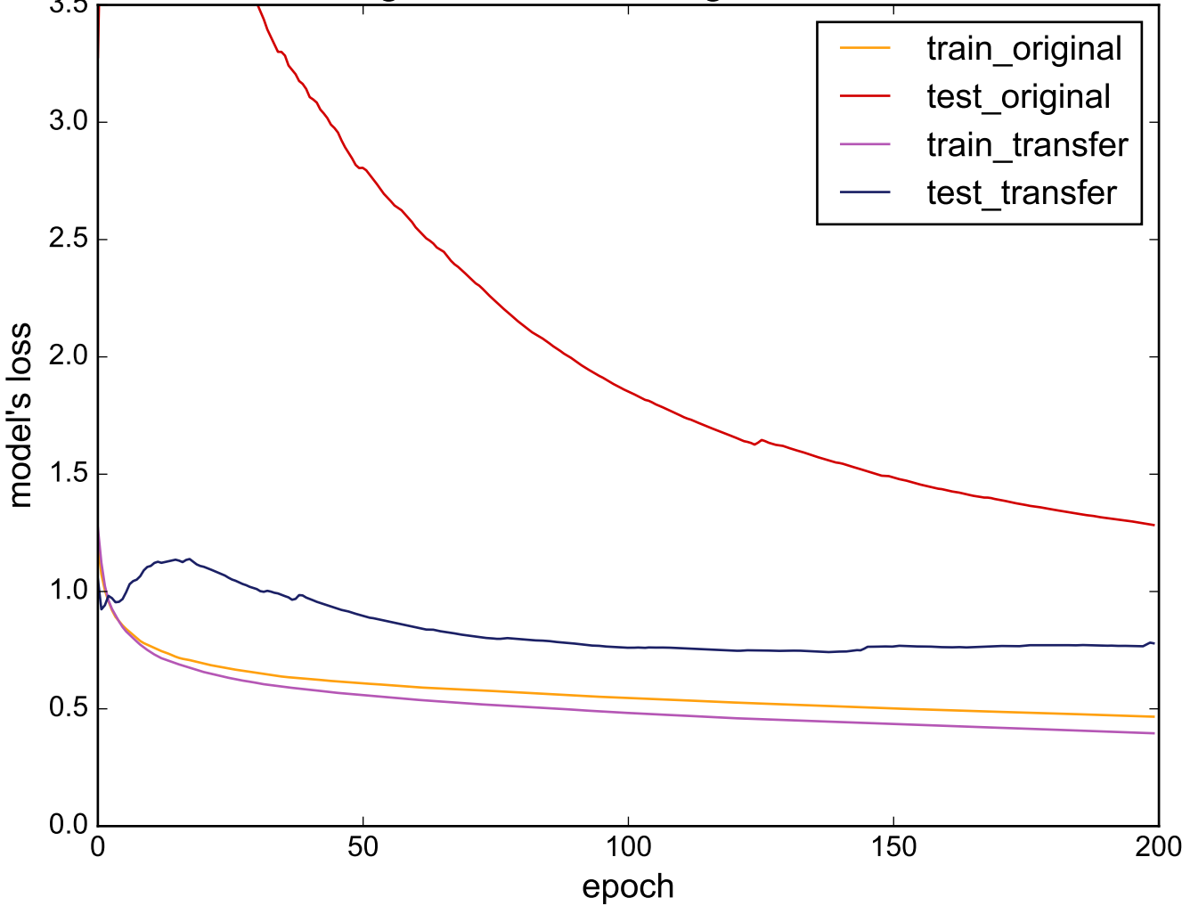
Source: ToeSegmentation1 - Target: ProximalPhalanxTW
