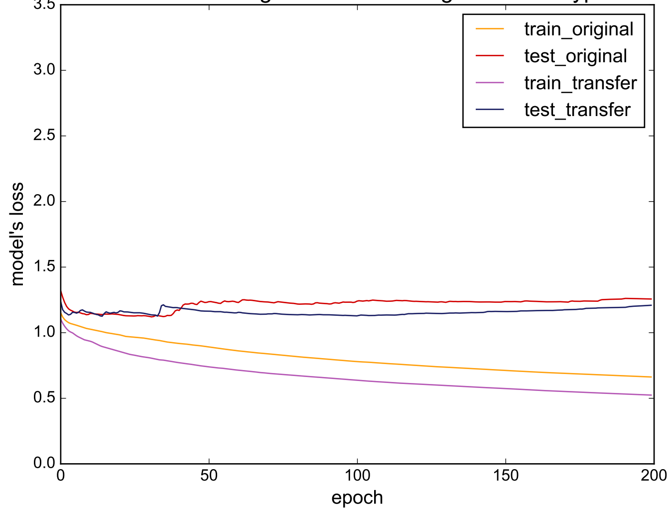
Source: ToeSegmentation1 - Target: ScreenType
