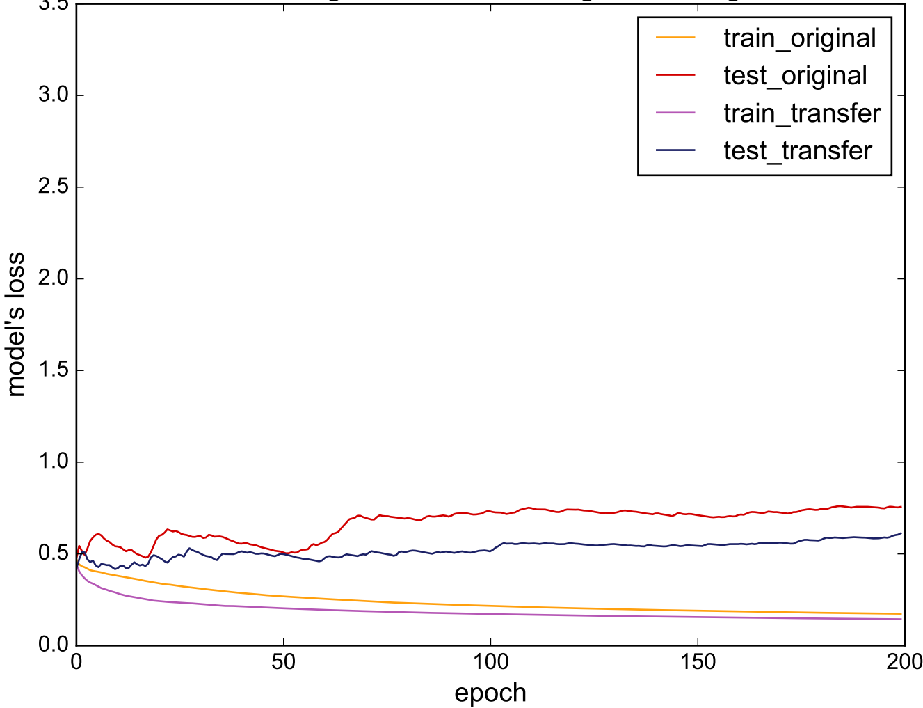
Source: ToeSegmentation1 - Target: StarLightCurves
