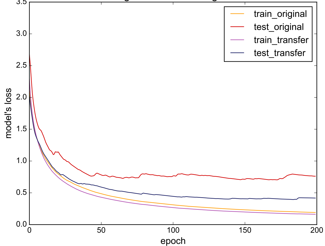
Source: ToeSegmentation1 - Target: SwedishLeaf
