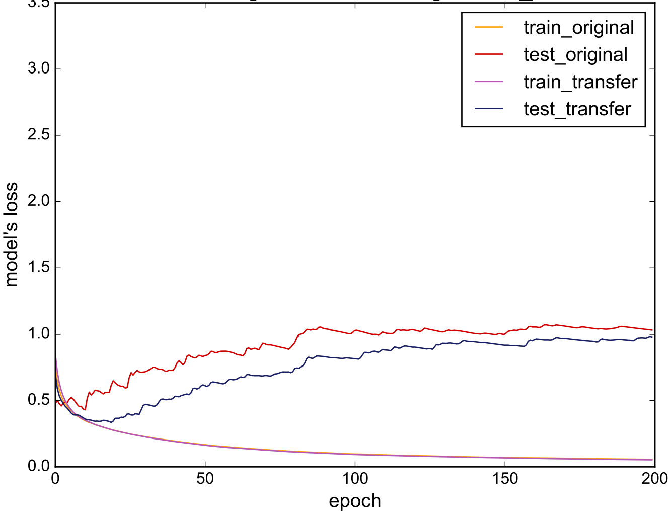
Source: ToeSegmentation1 - Target: Two_Patterns
