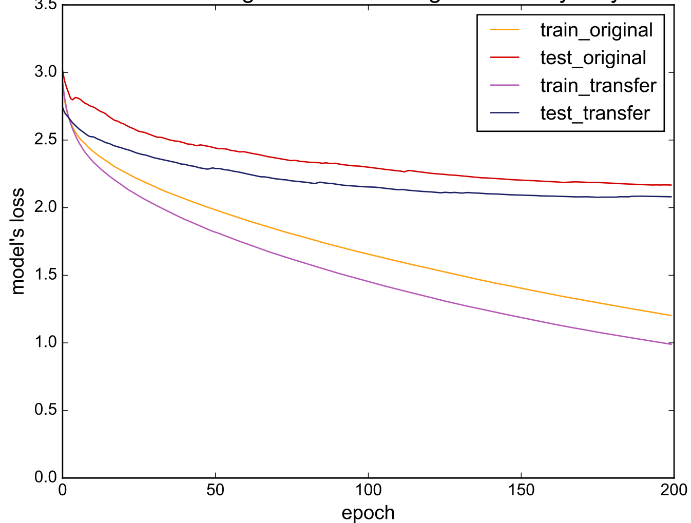
Source: ToeSegmentation1 - Target: WordsSynonyms
