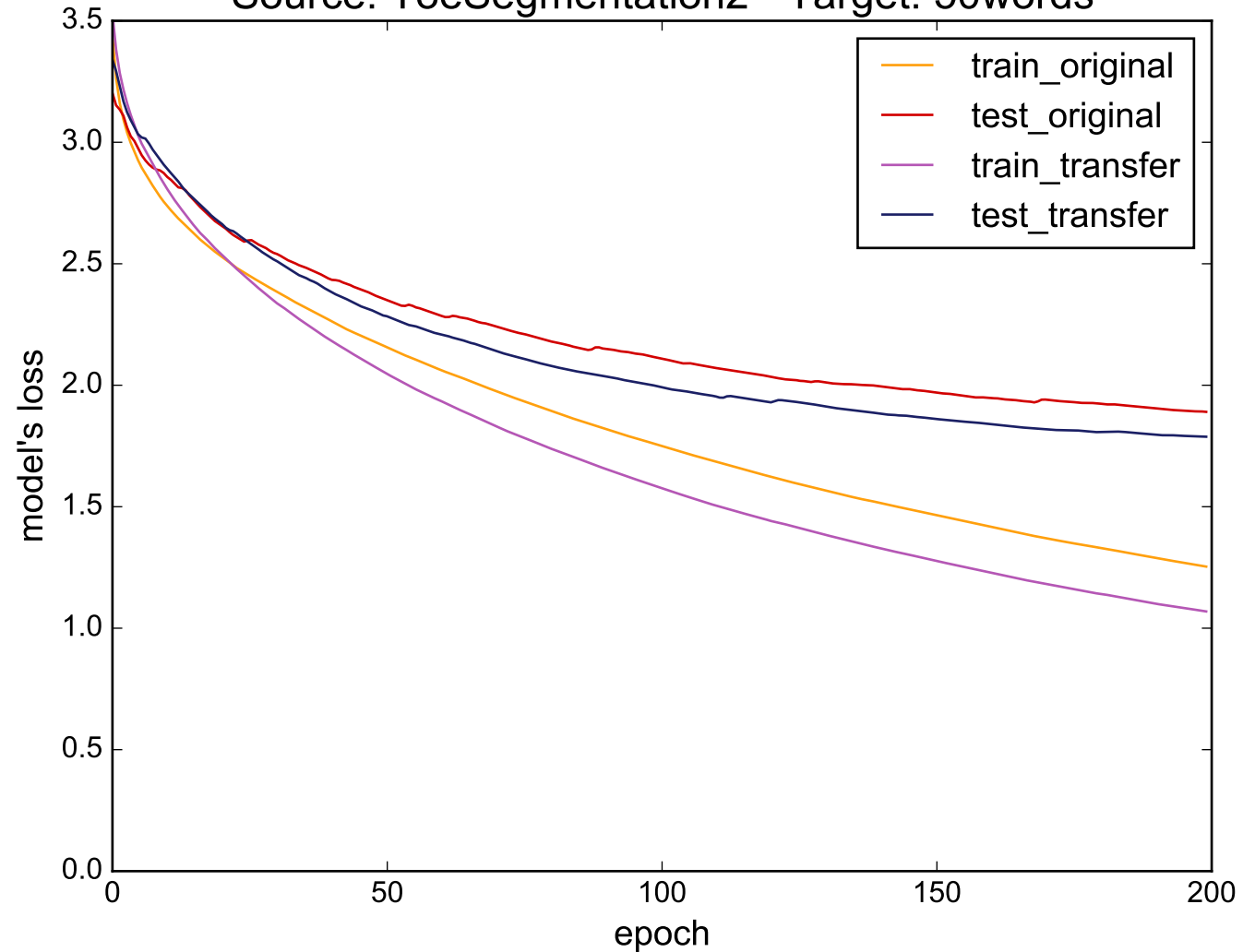
Source: ToeSegmentation2 - Target: 50words
