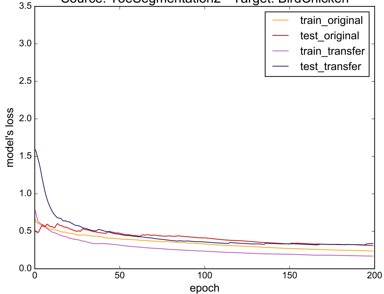
Source: ToeSegmentation2 - Target: BirdChicken
