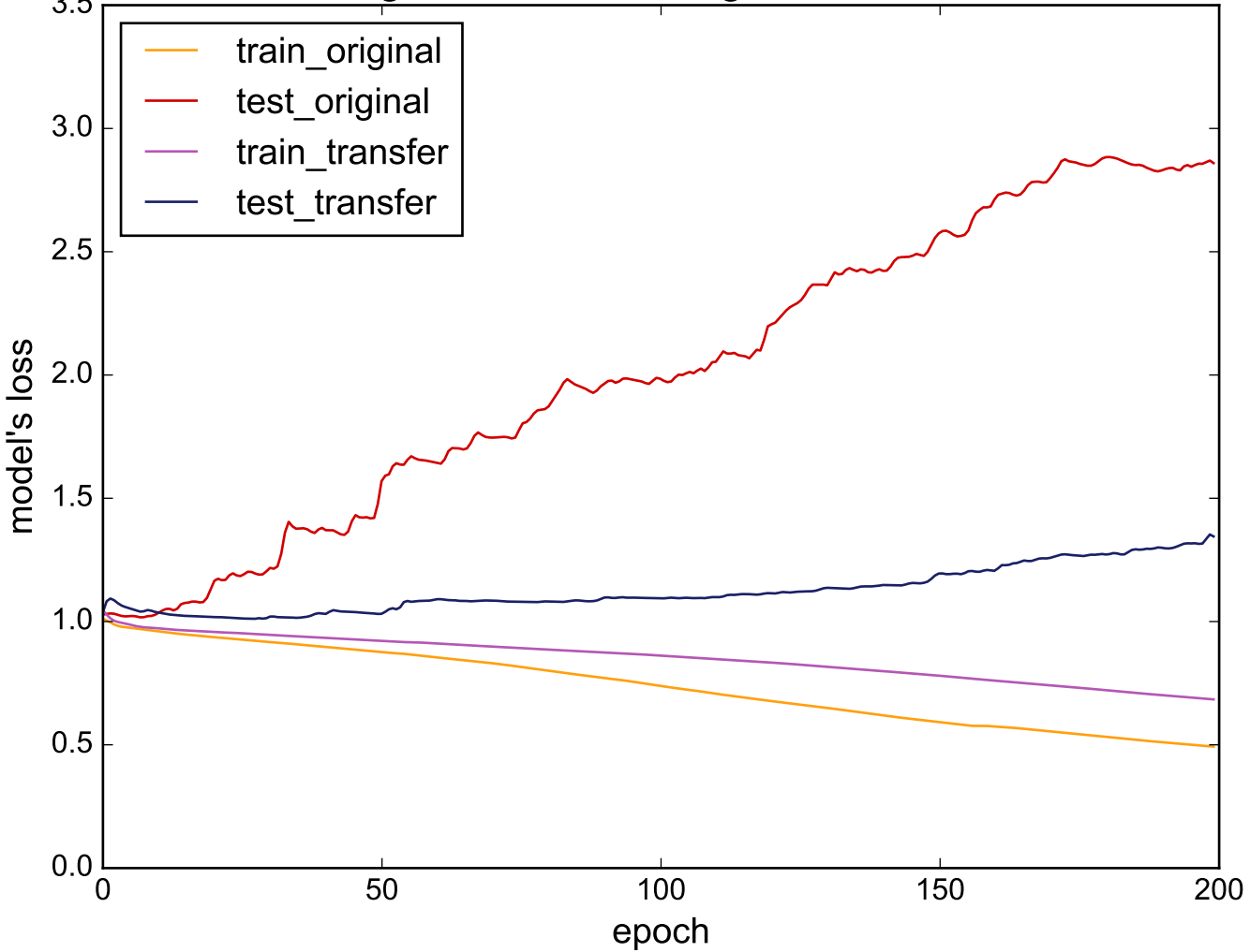
Source: ToeSegmentation2 - Target: ChlorineConcentration
