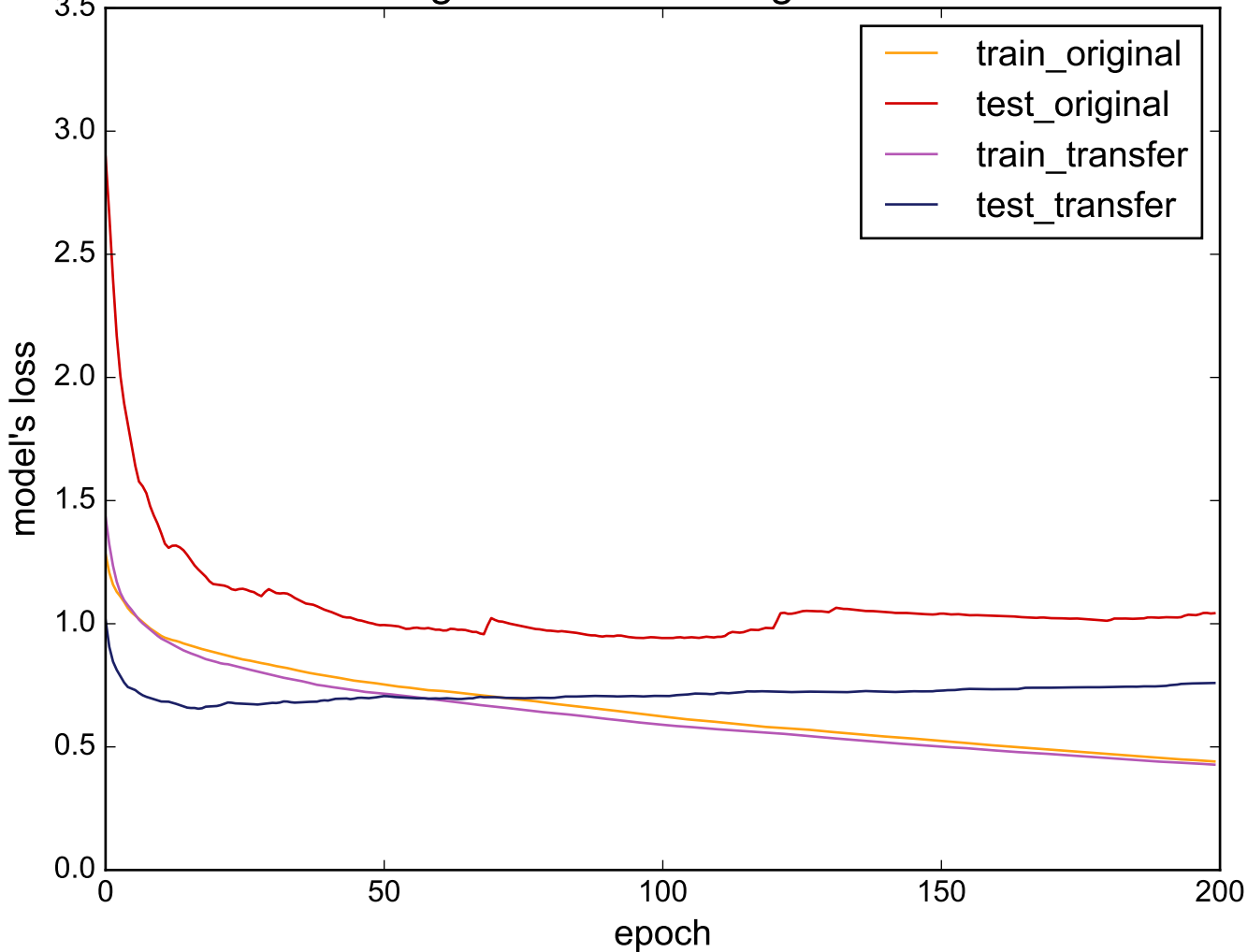
Source: ToeSegmentation2 - Target: DistalPhalanxTW
