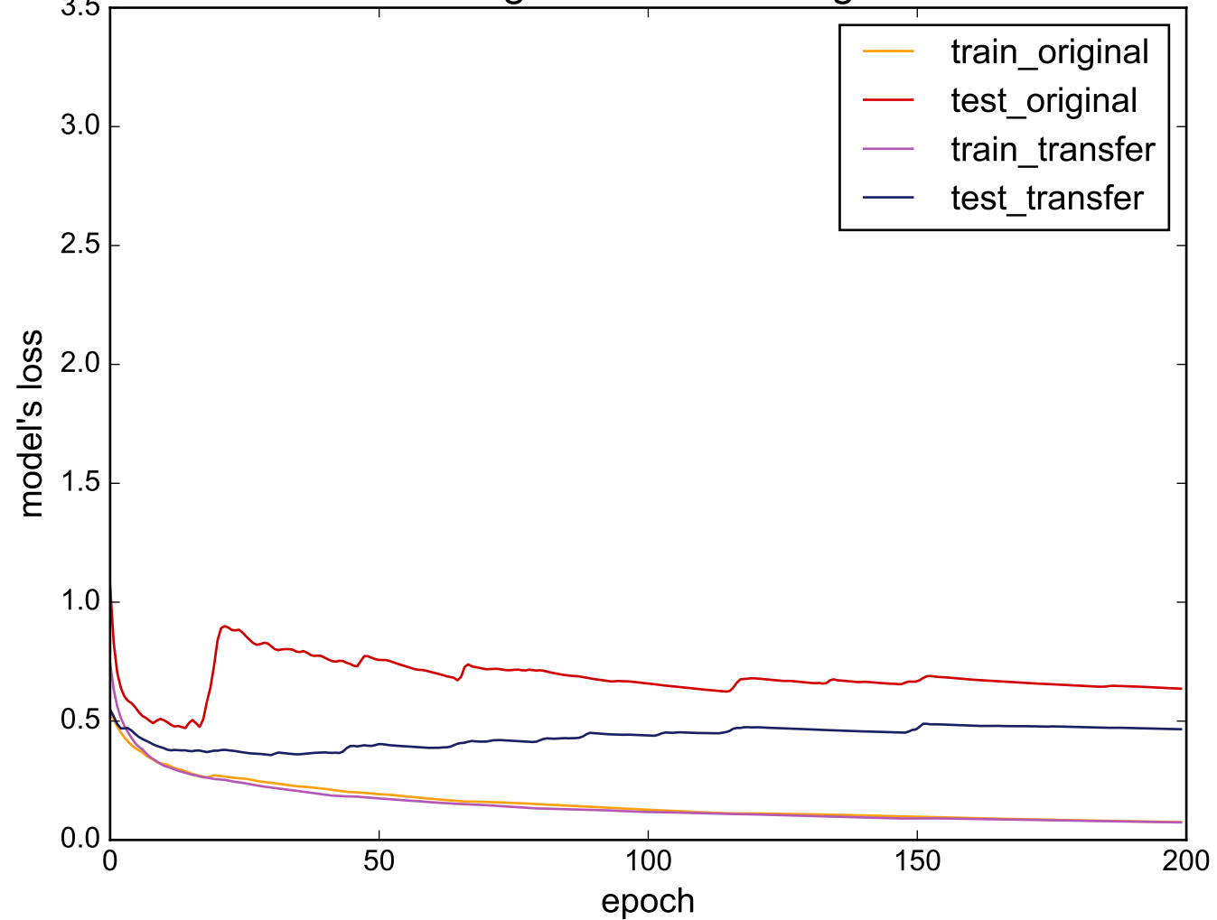
Source: ToeSegmentation2 - Target: ECG200
